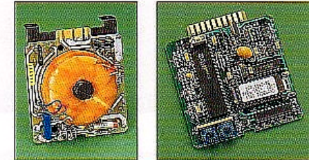
Replaceable plug-in circuit cards simplify field repair of the TF-3AC flasher/lampchanger. Left, power control circuit. Right, flash code timer.
